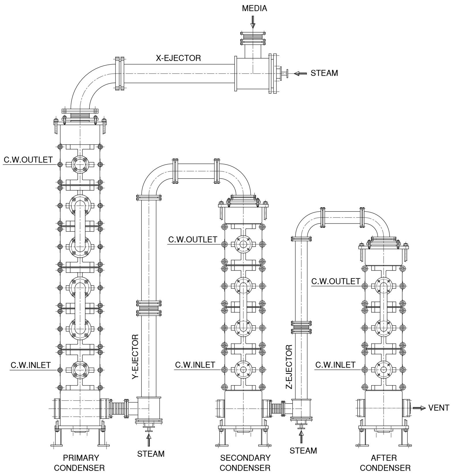
THREE STAGE EJECTOR SYSTEM-GRAPHITE
